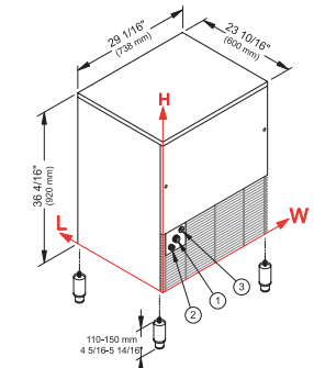
Adjustable feet 4 5/16" – 5 14/16"
