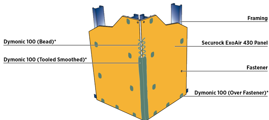
Fig. 1 : Outside corner
