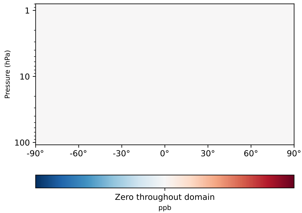
gcc-4x5-1Mon-14.7.0-alpha.10 - gcc-4x5-1Mon-14.7.0-alpha.9 (Ref) 4.0x5.0
