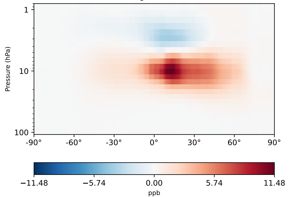
gchp-c24-1Mon-14.7.0-alpha.9_ - gchp-c24-1Mon-14.7.0-alpha.8 (Dev) 1x1.25 regridded from c24
