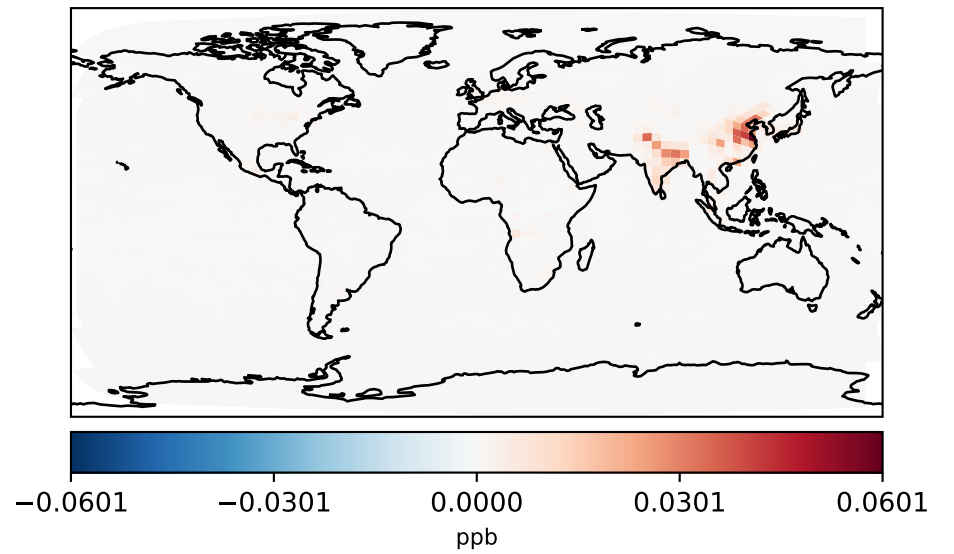
gchp-c24-1Mon-14.7.0-alpha.9_-_gchp-c24-1Mon-14.7.0-alpha.8 (Dev) c24
