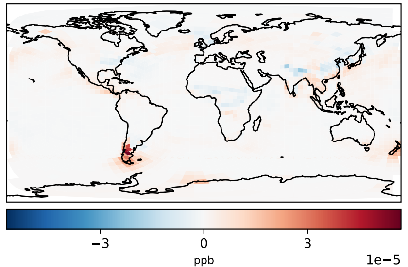
gchp-c24-1Mon-14.7.0-alpha.9_-_gchp-c24-1Mon-14.7.0-alpha.8 (Dev) c24
