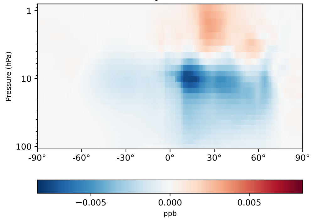
gchp-c24-1Mon-14.7.0-alpha.9_-gchp-c24-1Mon-14.7.0-alpha.8 (Dev) 1x1.25 regridged from c24
