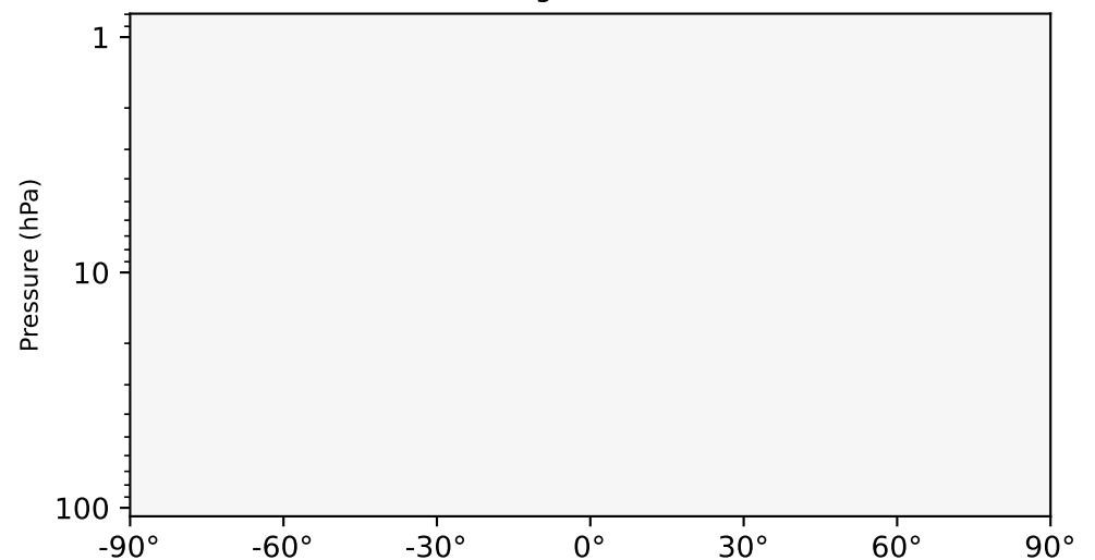
gchp-c24-1Mon-14.7.0-alpha.8 - gchp-c24-1Mon-14.7.0-alpha.7 (Dev) 1x1.25 regridded from c24
