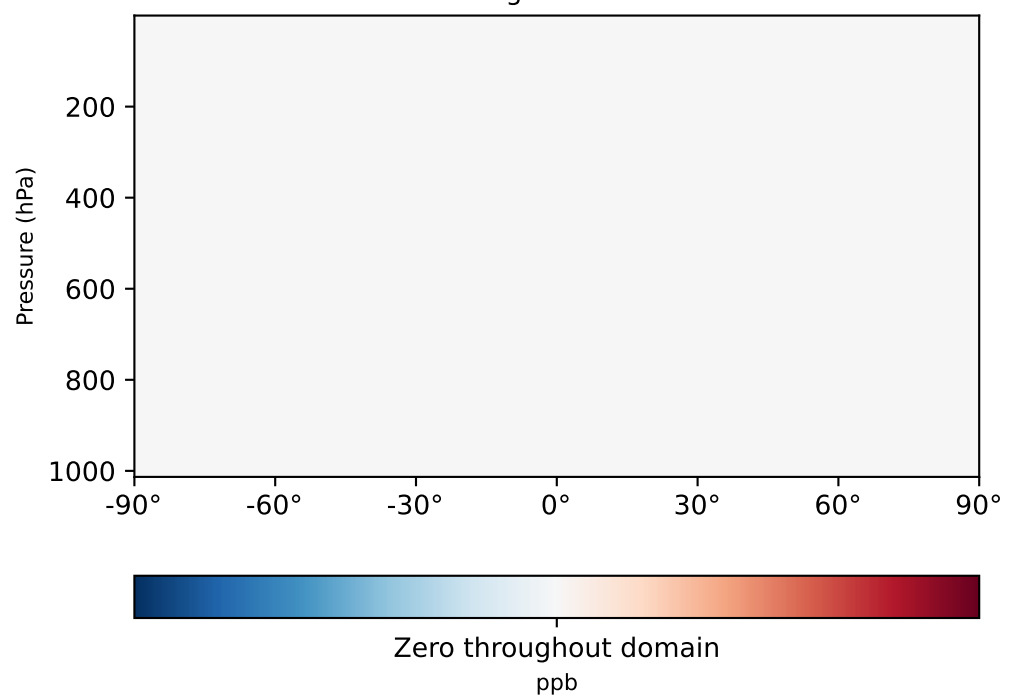
gchp-c24-1Mon-14.7.0-alpha.7 - gchp-c24-1Mon-14.7.0-alpha.6 (Dev) 1x1.25 regridged from c24
