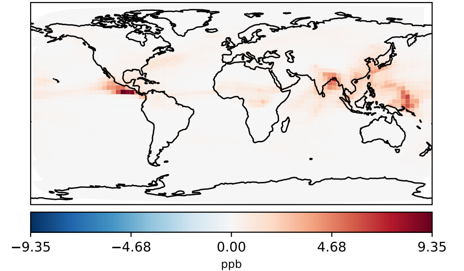
gchp-c24-1Mon-14.7.0-alpha.6_-_gchp-c24-1Mon-14.7.0-alpha.5 (Dev) c24
