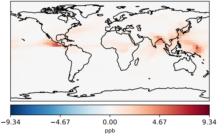
gcc-4x5-1Mon-14.7.0-alpha.6_-_gcc-4x5-1Mon-14.7.0-alpha.5 (Ref) 4.0x5.0
