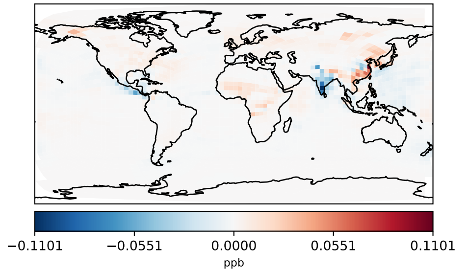
gchp-c24-1Mon-14.7.0-alpha.6_-_gchp-c24-1Mon-14.7.0-alpha.5 (Dev) c24
