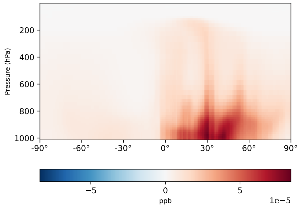
gchp-c24-1Mon-14.7.0-alpha.6_- gchp-c24-1Mon-14.7.0-alpha.5 (Dev) 1x1.25 regridged from c24
