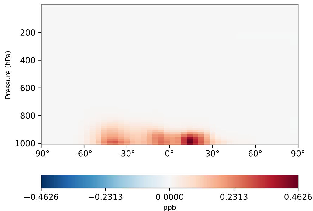
gcc-4x5-1Mon-14.7.0-alpha.6_-gcc-4x5-1Mon-14.7.0-alpha.5 (Ref) 4.0x5.0
