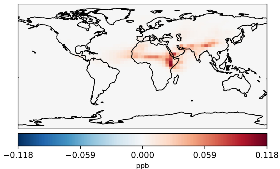
gcc-4x5-1Mon-14.7.0-alpha.6_-_gcc-4x5-1Mon-14.7.0-alpha.5 (Ref) 4.0x5.0
