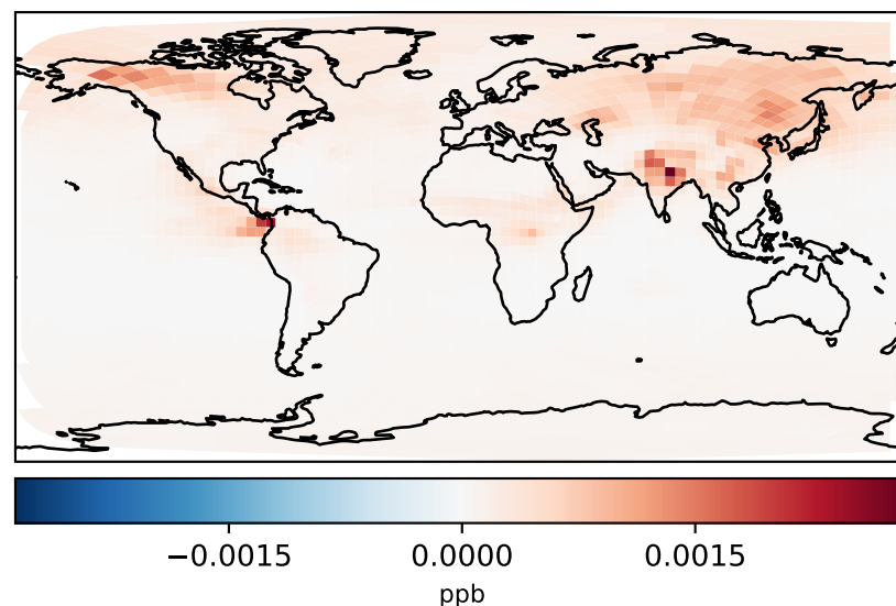
gchp-c24-1Mon-14.7.0-alpha.6_-_gchp-c24-1Mon-14.7.0-alpha.5 (Dev) c24
