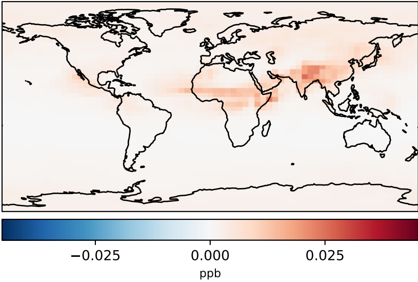
gcc-4x5-1Mon-14.7.0-alpha.6_-_gcc-4x5-1Mon-14.7.0-alpha.5 (Ref) 4.0x5.0
