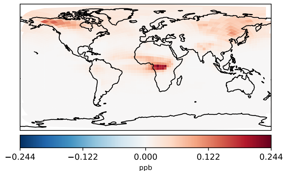
gchp-c24-1Mon-14.7.0-alpha.6_-_gchp-c24-1Mon-14.7.0-alpha.5 (Dev) c24
