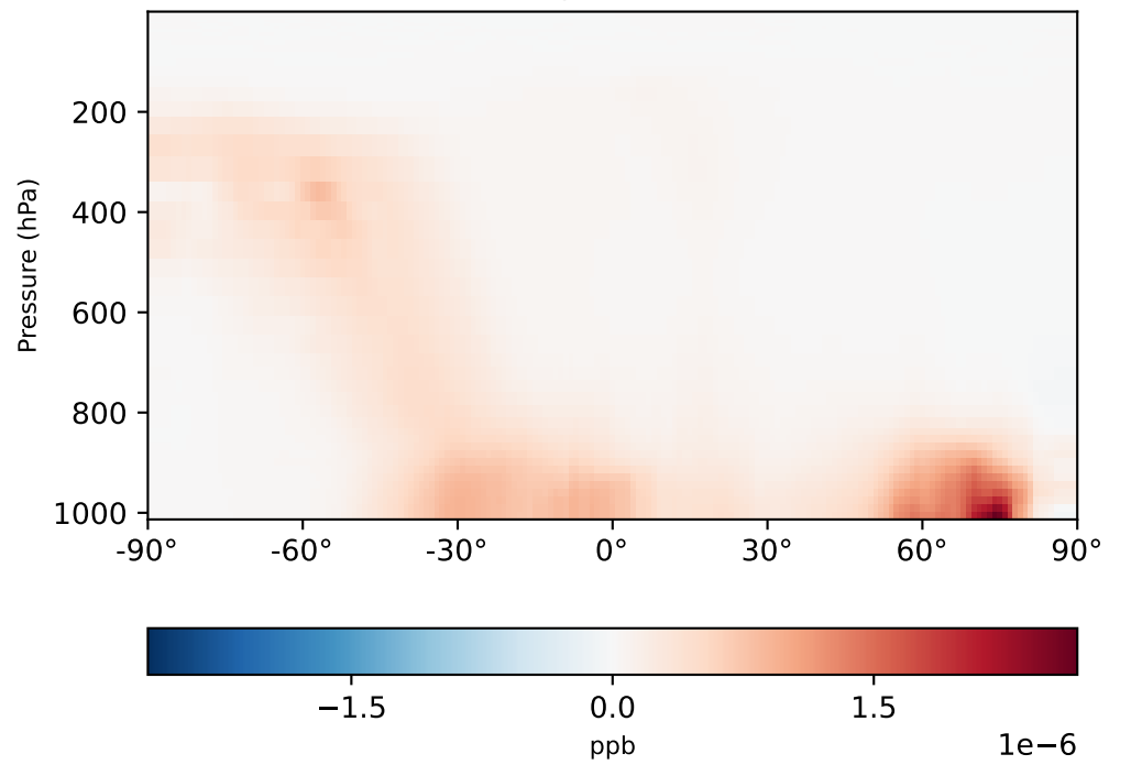
gchp-c24-1Mon-14.7.0-alpha.5_ - gchp-c24-1Mon-14.7.0-alpha.4 (Dev) 1x1.25 regridded from c24
