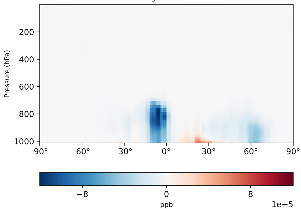
gchp-c24-1Mon-14.7.0-alpha.5_ - gchp-c24-1Mon-14.7.0-alpha.4 (Dev) 1x1.25 regridded from c24
