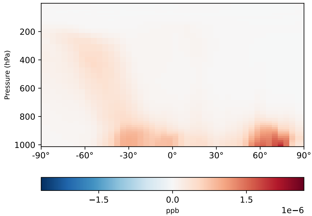
gcc-4x5-1Mon-14.7.0-alpha.5_ - gcc-4x5-1Mon-14.7.0-alpha.4 (Ref) 4.0x5.0
