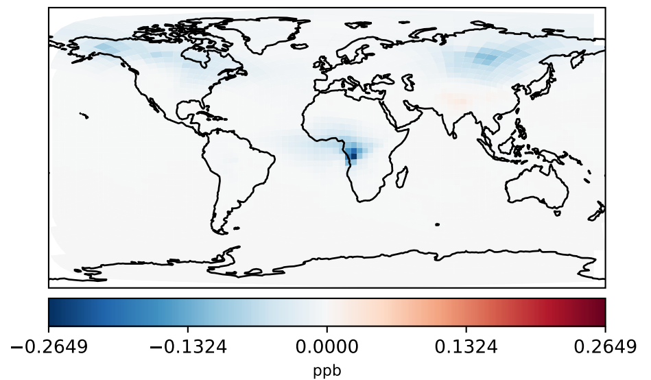
gchp-c24-1Mon-14.7.0-alpha.5_-_gchp-c24-1Mon-14.7.0-alpha.4 (Dev) c24
