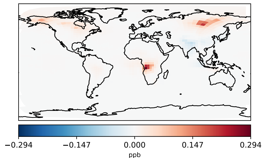
gchp-c24-1Mon-14.7.0-alpha.5_-_gchp-c24-1Mon-14.7.0-alpha.4 (Dev) c24
