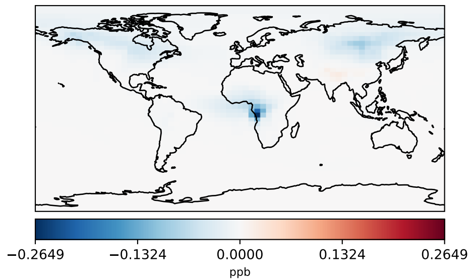
gcc-4x5-1Mon-14.7.0-alpha.5_-_gcc-4x5-1Mon-14.7.0-alpha.4 (Ref) 4.0x5.0
