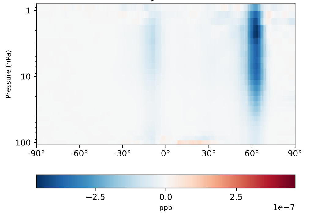
gchp-c24-1Mon-14.7.0-alpha.5_ - gchp-c24-1Mon-14.7.0-alpha.4 (Dev) 1x1.25 regridded from c24
