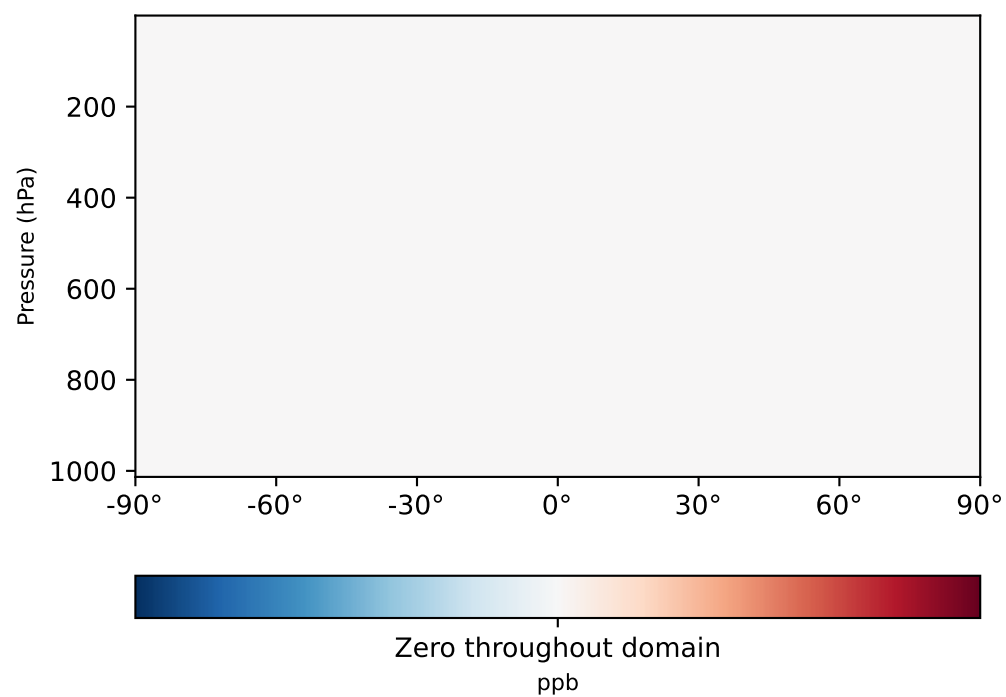
gcc-4x5-1Mon-14.7.0-alpha.4 - gcc-4x5-1Mon-14.7.0-alpha.3 (Ref) 4.0x5.0
