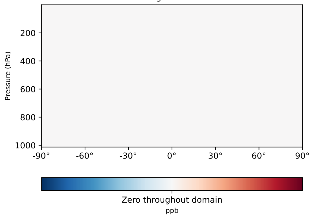
gchp-c24-1Mon-14.7.0-alpha.4 - gchp-c24-1Mon-14.7.0-alpha.3 (Dev) 1x1.25 regridded from c24
