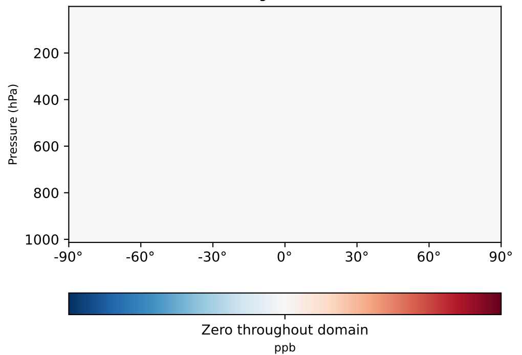
gchp-c24-1Mon-14.7.0-alpha.18_ - gchp-c24-1Mon-14.7.0-alpha.17 (Dev) 1x1.25 regridded from c24
