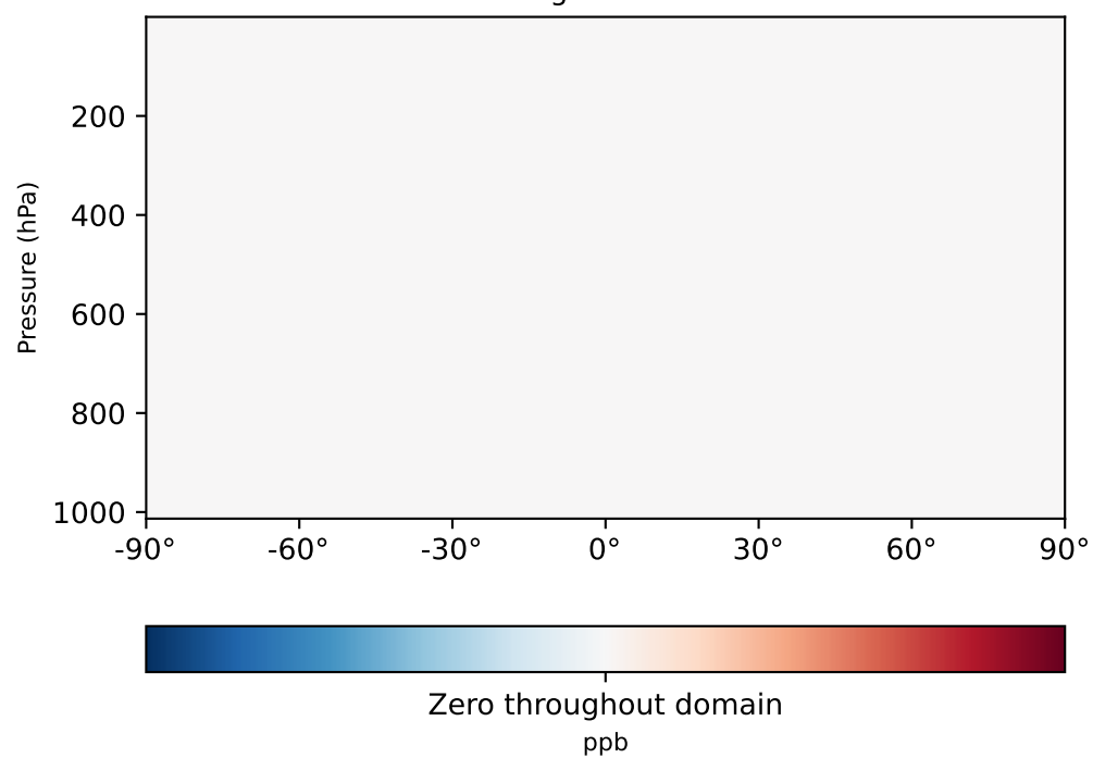
gchp-c24-1Mon-14.7.0-alpha.18_ - gchp-c24-1Mon-14.7.0-alpha.17 (Dev) 1x1.25 regridded from c24
