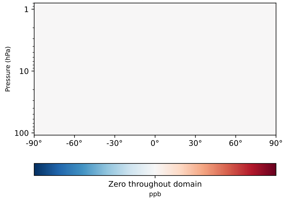
gchp-c24-1Mon-14.7.0-alpha.15_ - gchp-c24-1Mon-14.7.0-alpha.14 (Dev) 1x1.25 regridded from c24
