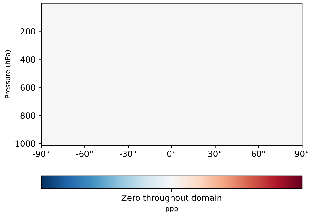
gchp-c24-1Mon-14.7.0-alpha.15_ - gchp-c24-1Mon-14.7.0-alpha.14 (Dev) 1x1.25 regridded from c24
