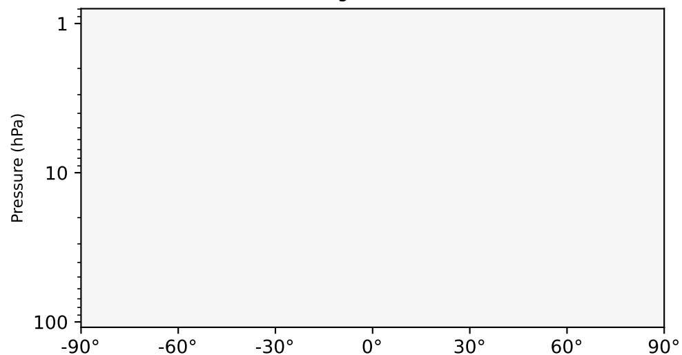
gchp-c24-1Mon-14.7.0-alpha.14 - gchp-c24-1Mon-14.7.0-alpha.13 (Dev) 1x1.25 regridded from c24
