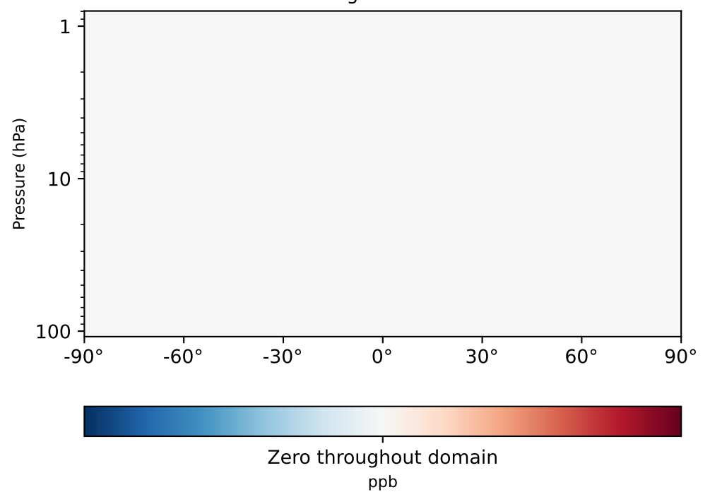
gchp-c24-1Mon-14.7.0-alpha.13_ - gchp-c24-1Mon-14.7.0-alpha.12 (Dev) 1x1.25 regridded from c24
