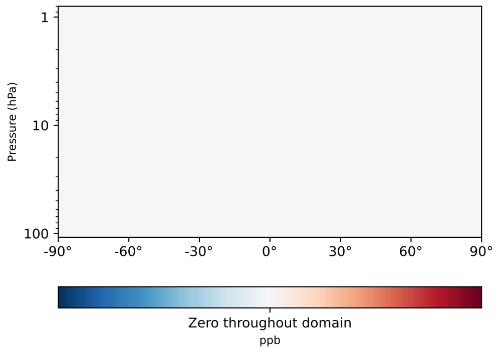
gcc-4x5-1Mon-14.7.0-alpha.13_ - gcc-4x5-1Mon-14.7.0-alpha.12 (Ref) 4.0x5.0
