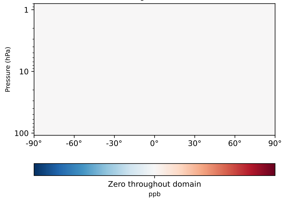
gchp-c24-1Mon-14.7.0-alpha.13_ - gchp-c24-1Mon-14.7.0-alpha.12 (Dev) 1x1.25 regridded from c24
