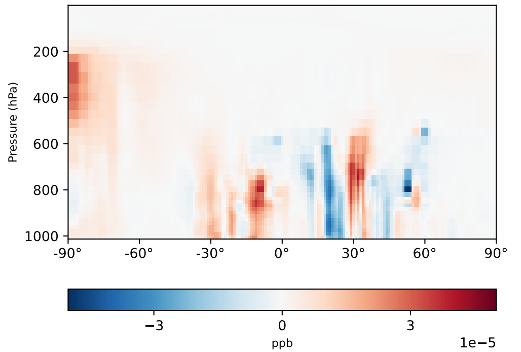
gchp-c24-1Mon-14.7.0-alpha.12_ - gchp-c24-1Mon-14.7.0-alpha.11 (Dev) 1x1.25 regridded from c24
