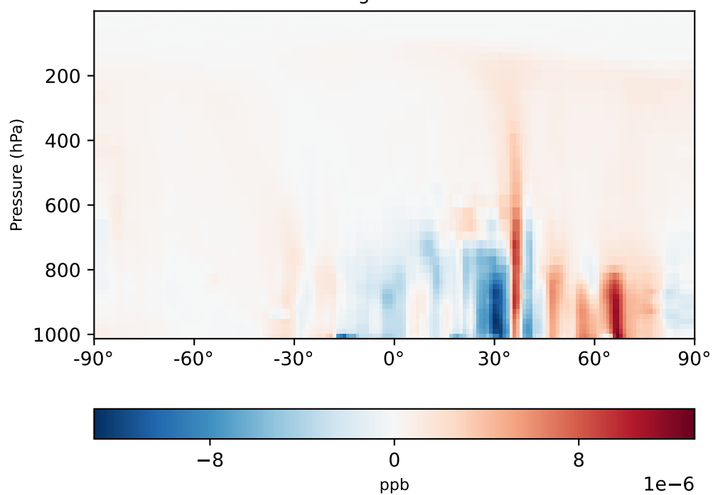
gchp-c24-1Mon-14.7.0-alpha.12_ - gchp-c24-1Mon-14.7.0-alpha.11 (Dev) 1x1.25 regridded from c24
