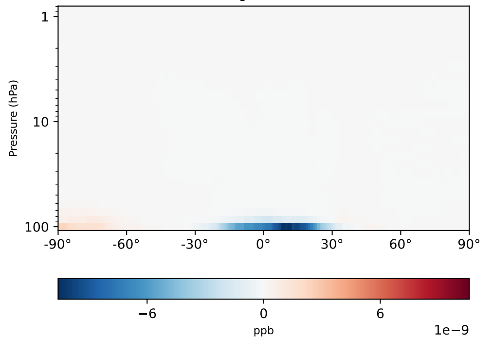
gchp-c24-1Mon-14.7.0-alpha.12_-gchp-c24-1Mon-14.7.0-alpha.11 (Dev) 1x1.25 regridded from c24
