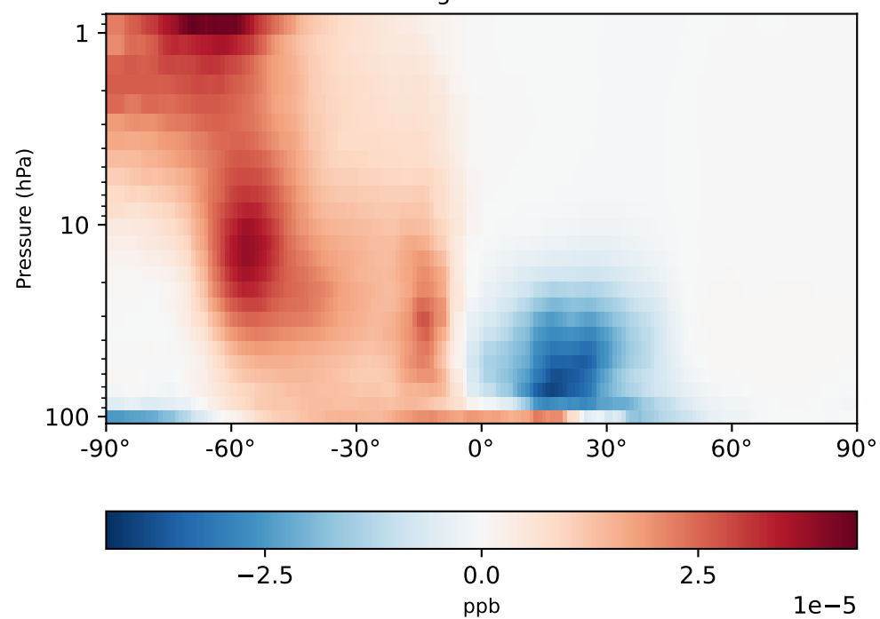
gchp-c24-1Mon-14.7.0-alpha.12_- gchp-c24-1Mon-14.7.0-alpha.11 (Dev) 1x1.25 regridged from c24
