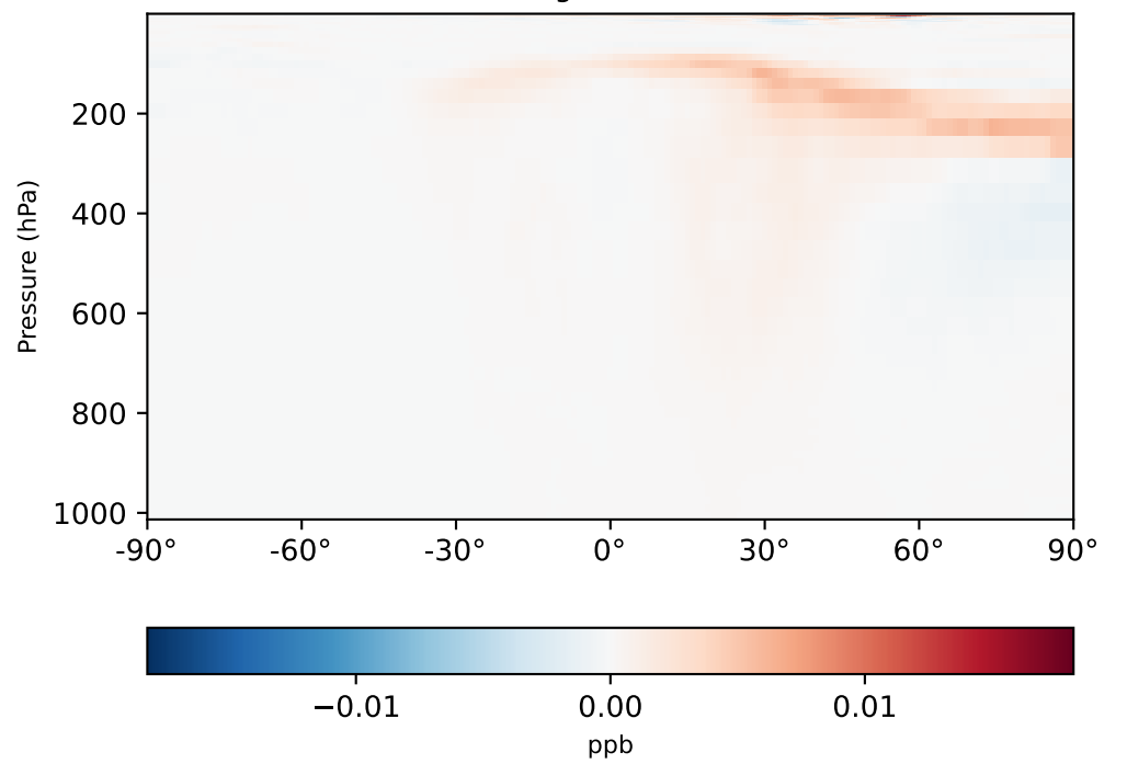
gchp-c24-1Mon-14.7.0-alpha.11_ - gchp-c24-1Mon-14.7.0-alpha.10 (Dev) 1x1.25 regridded from c24
