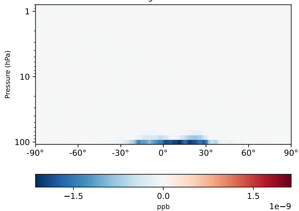
gchp-c24-1Mon-14.7.0-alpha.11_ - gchp-c24-1Mon-14.7.0-alpha.10 (Dev) 1x1.25 regridded from c24
