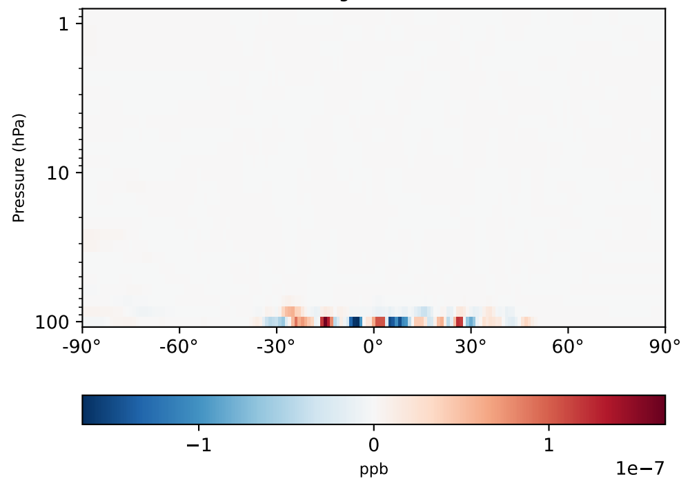
gchp-c24-1Mon-14.7.0-alpha.11_ - gchp-c24-1Mon-14.7.0-alpha.10 (Dev) 1x1.25 regridded from c24
