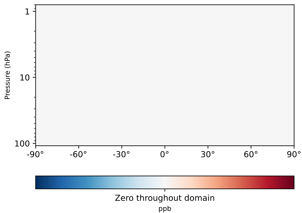
gcc-4x5-1Mon-14.7.0-alpha.11_ - gcc-4x5-1Mon-14.7.0-alpha.10 (Ref) 4.0x5.0
