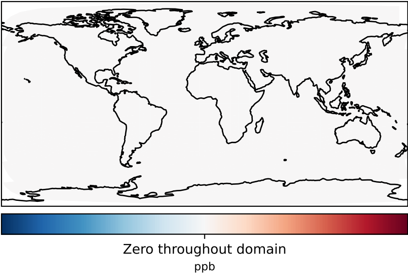
gchp-c24-1Mon-14.7.0-alpha.3_-_gchp-c24-1Mon-14.6.3 (Dev) c24
