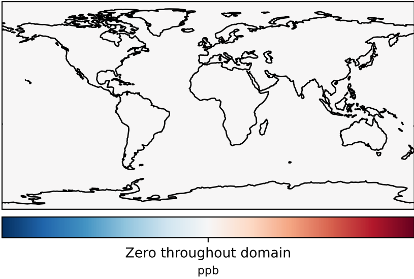
gcc-4x5-1Mon-14.7.0-alpha.3_-_gcc-4x5-1Mon-14.6.3 (Ref) 4.0x5.0
