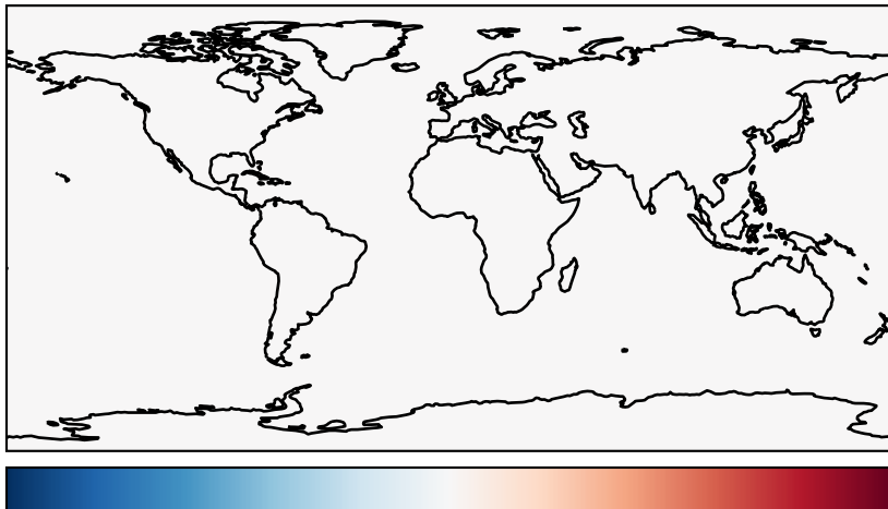
gcc-4x5-1Mon-14.7.0-alpha.3_-_gcc-4x5-1Mon-14.6.3 (Ref) 4.0x5.0
