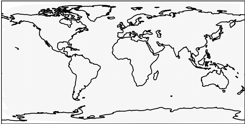
gchp-c24-1Mon-14.7.0-alpha.3_-_gchp-c24-1Mon-14.6.3 (Dev) c24
