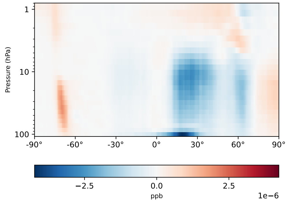
gchp-c24-1Mon-14.7.0-alpha.17 - gchp-c24-1Mon-14.6.3 (Dev) 1x1.25 regridded from c24
