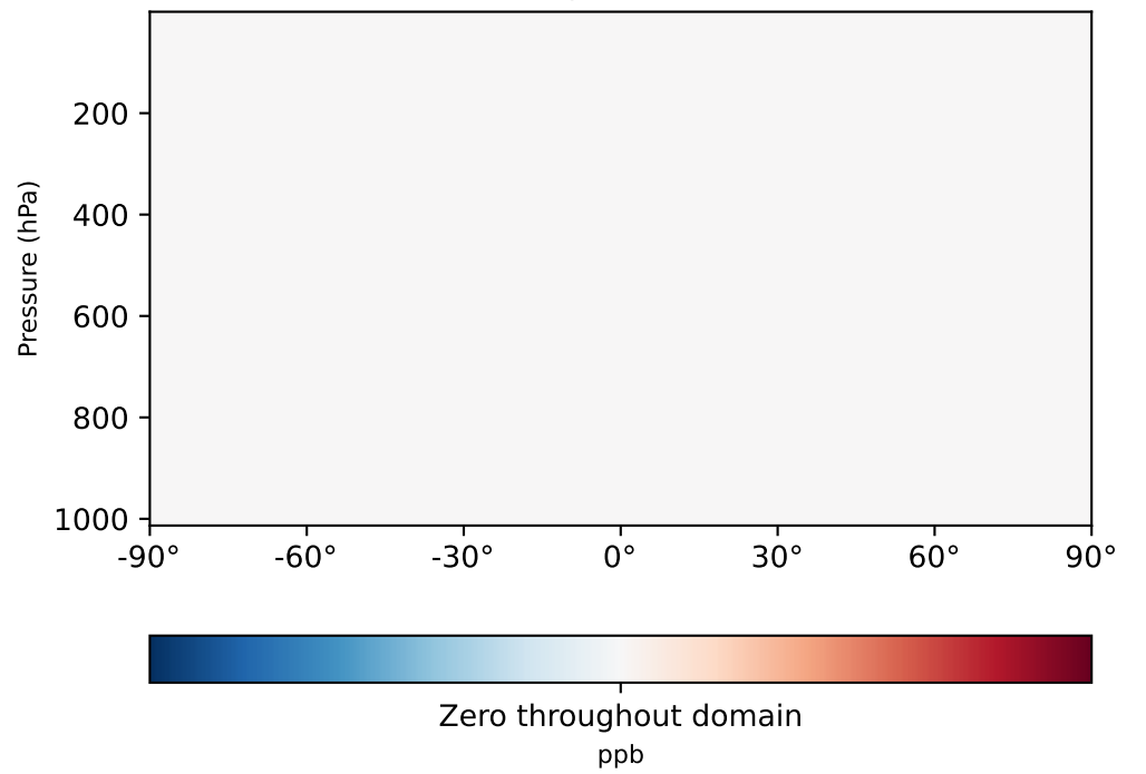
gchp-c24-1Mon-14.7.0-alpha.0 - _gchp-c24-1Mon-14.6.2 (Dev) 1x1.25 regridded from c24
