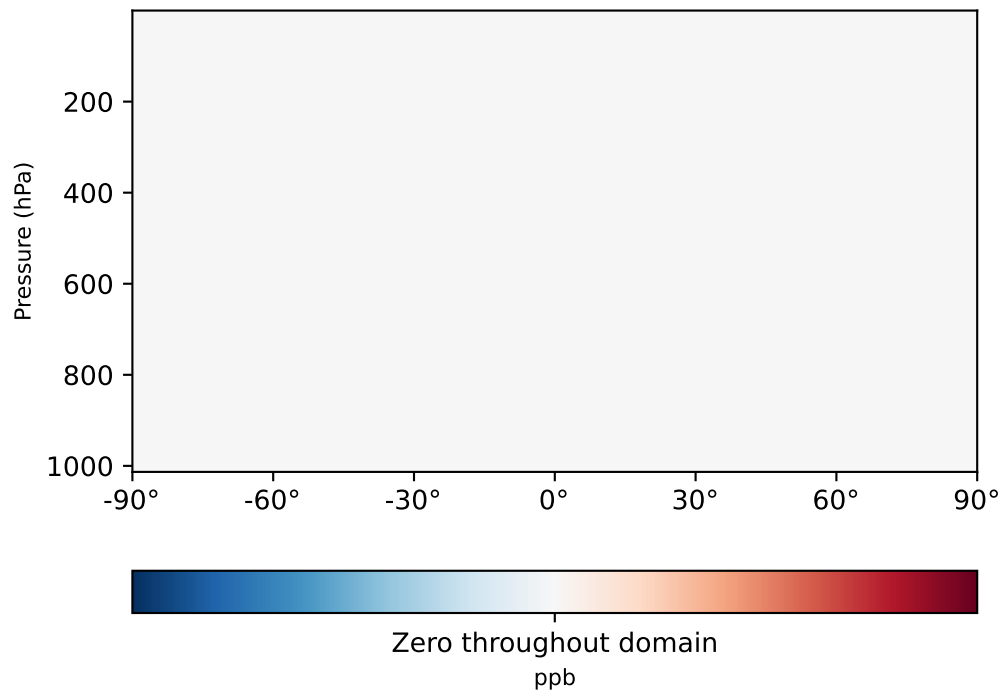
gcc-4x5-1Mon-14.7.0-alpha.0 - _gcc-4x5-1Mon-14.6.2 (Ref) 4.0x5.0
