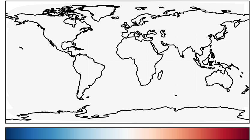
gchp-c24-1Mon-14.7.0-alpha.0_-_gchp-c24-1Mon-14.6.2 (Dev) c24
