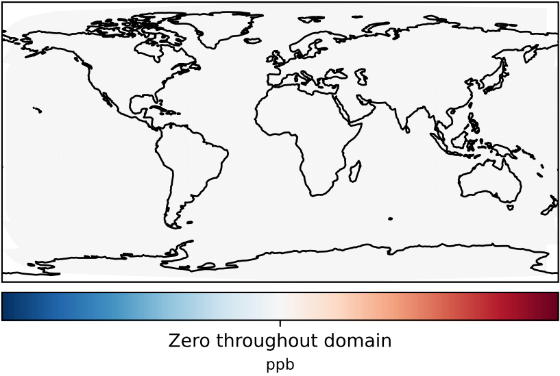
gchp-c24-1Mon-14.7.0-alpha.0_-_gchp-c24-1Mon-14.6.2 (Dev) c24
