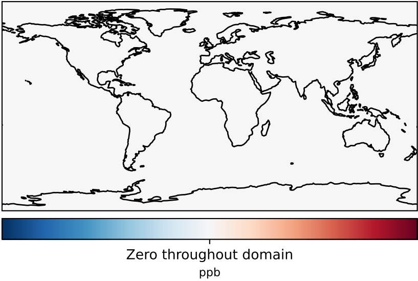
gcc-4x5-1Mon-14.7.0-alpha.0_-_gcc-4x5-1Mon-14.6.2 (Ref) 4.0x5.0
