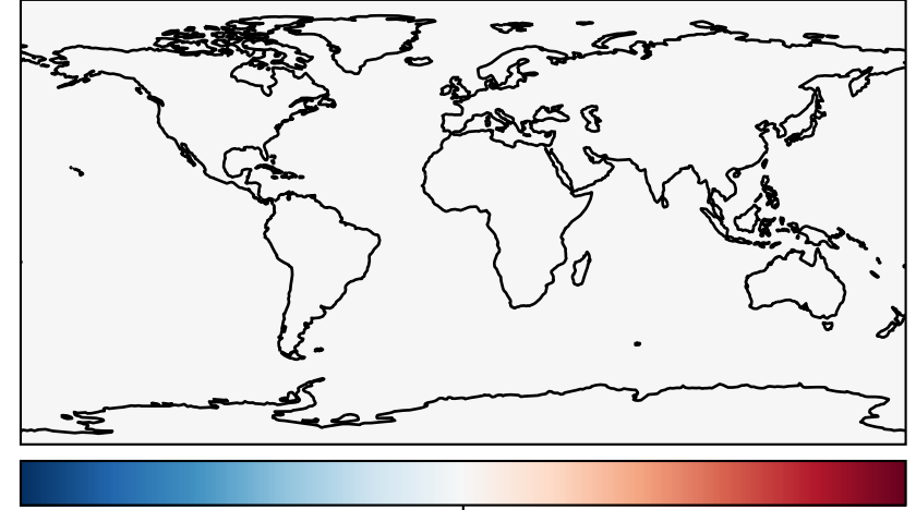
Difference (1x1.25), Restricted Range [5%,95%] GCHP_dev / GCHP_ref - GCC_dev / GCC_ref
