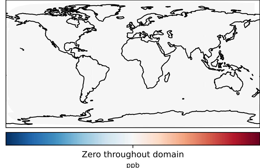
gchp-c24-1Mon-14.7.0-alpha.0_-_gchp-c24-1Mon-14.6.2 (Dev) c24
