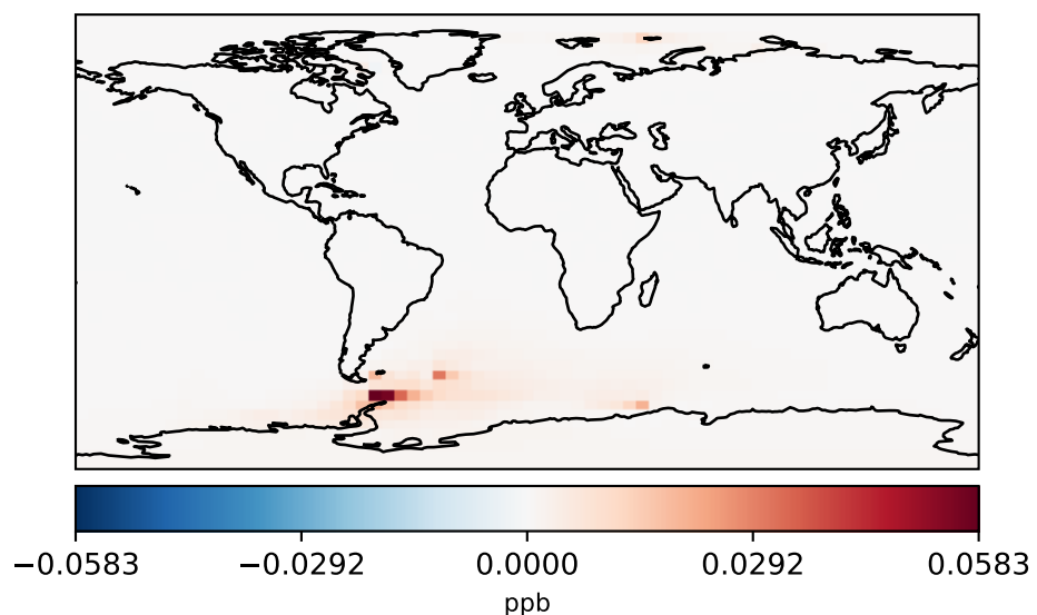
gcc-4x5-1Mon-14.6.0-alpha.6_-_gcc-4x5-1Mon-14.6.0-alpha.5 (Ref) 4.0x5.0
