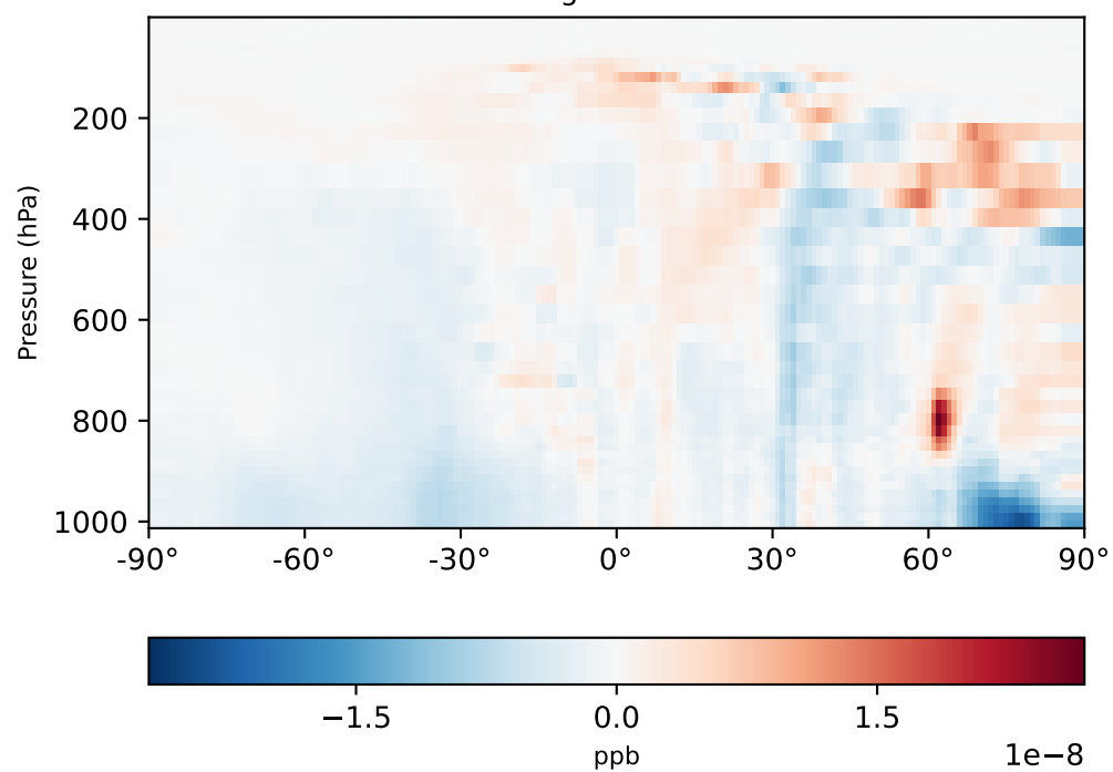
gchp-c24-1Mon-14.6.0-alpha.6_- gchp-c24-1Mon-14.6.0-alpha.5 (Dev) 1x1.25 regrided from c24
