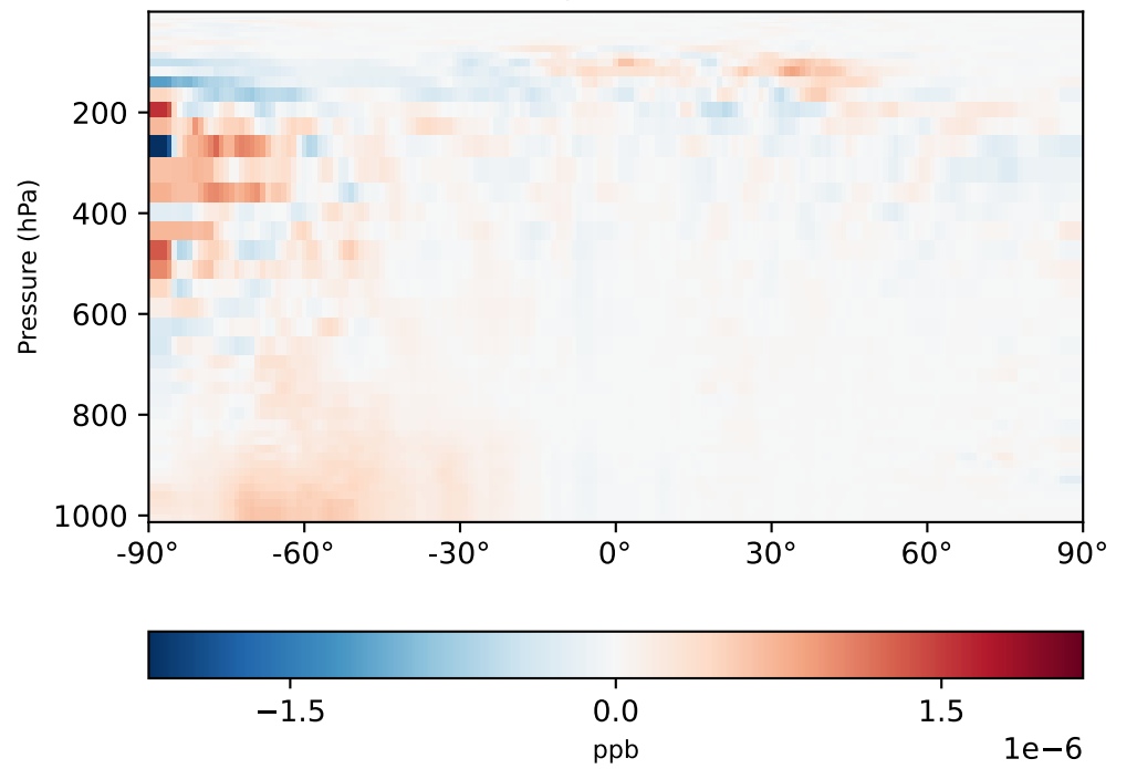
gchp-c24-1Mon-14.6.0-alpha.6_- gchp-c24-1Mon-14.6.0-alpha.5 (Dev) 1x1.25 regridged from c24
