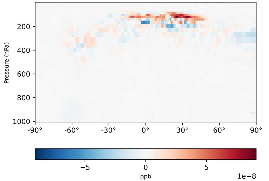
gchp-c24-1Mon-14.6.0-alpha.6_- gchp-c24-1Mon-14.6.0-alpha.5 (Dev) 1x1.25 regridded from c24
