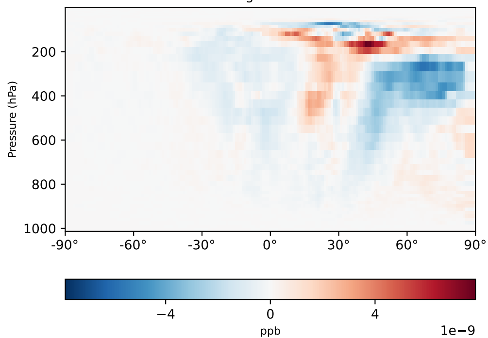
gchp-c24-1Mon-14.6.0-alpha.6_-gchp-c24-1Mon-14.6.0-alpha.5 (Dev) 1x1.25 regridded from c24
