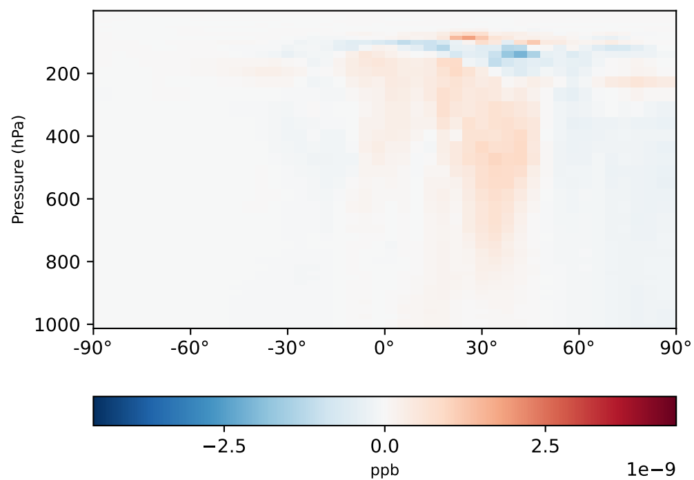
gcc-4x5-1Mon-14.6.0-alpha.6_-gcc-4x5-1Mon-14.6.0-alpha.5 (Ref) 4.0x5.0
