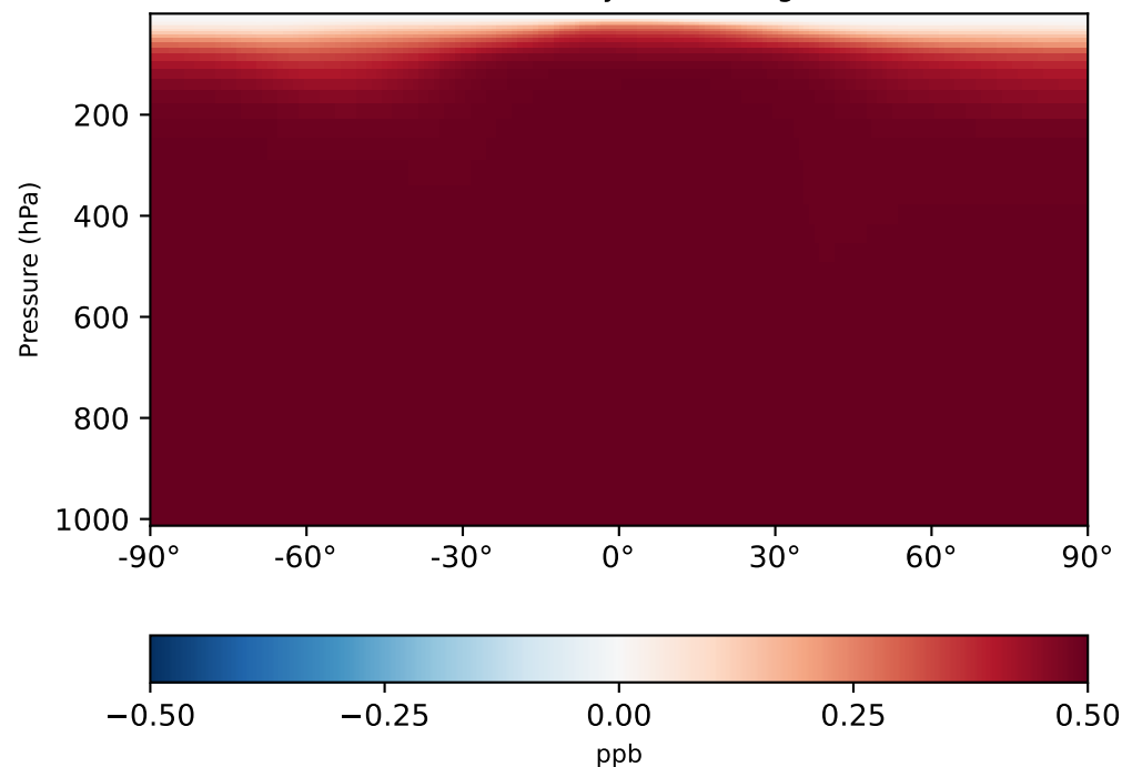
Difference (1x1.25) Dev - Ref, Dynamic Range
