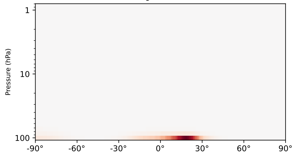
gchp-c24-1Mon-14.6.0-alpha.15_ - gchp-c24-1Mon-14.6.0-alpha.14 (Dev) 1x1.25 regridded from c24
