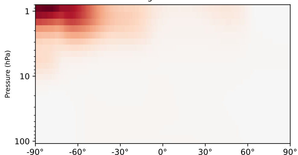
gchp-c24-1Mon-14.6.0-alpha.15_ - gchp-c24-1Mon-14.6.0-alpha.14 (Dev) 1x1.25 regridded from c24
