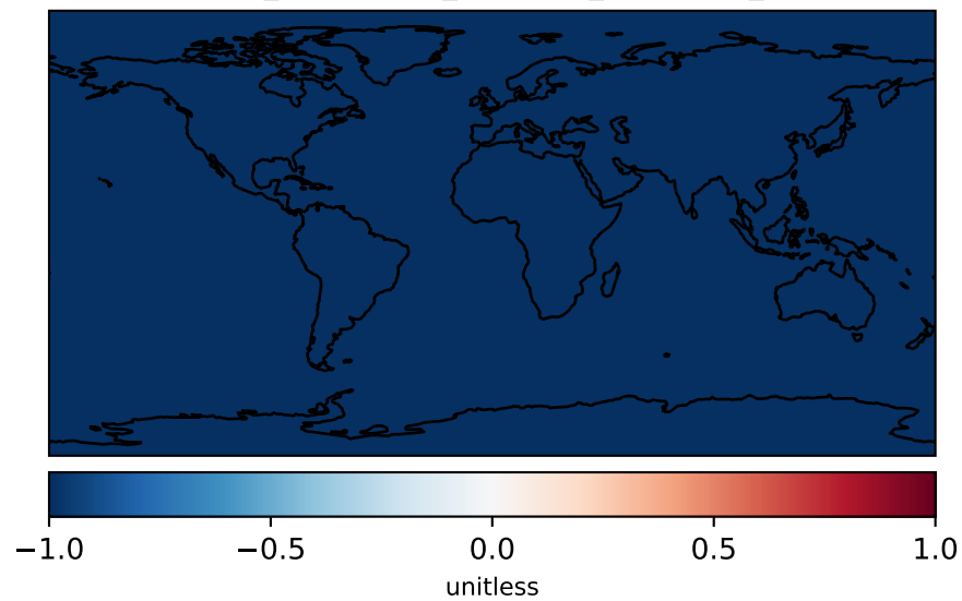
Difference (1x1.25), Dynamic Range \text{GCHP\_dev} / \text{GCHP\_ref} - \text{GCC\_dev} / \text{GCC\_ref}
