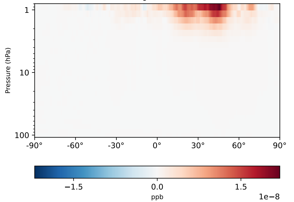
gchp-c24-1Mon-14.4.0-alpha.1 - gchp-c24-1Mon-14.4.0-alpha.0 (Dev) 1x1.25 regridded from c24
