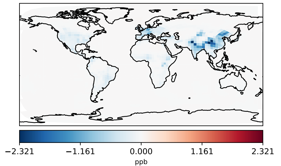
gchp-c24-1Mon-14.4.0-alpha.1 - gchp-c24-1Mon-14.4.0-alpha.0 (Dev) c24
