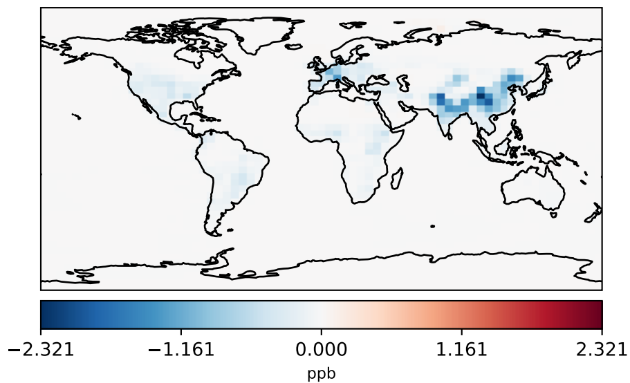
gcc-4x5-1Mon-14.4.0-alpha.1 - gcc-4x5-1Mon-14.4.0-alpha.0 (Ref) 4.0x5.0
