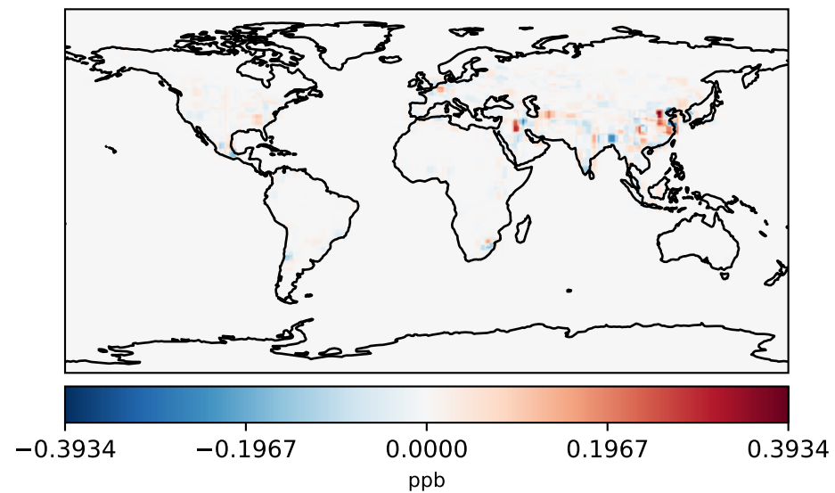
Difference (1x1.25) Dev - Ref, Dynamic Range
