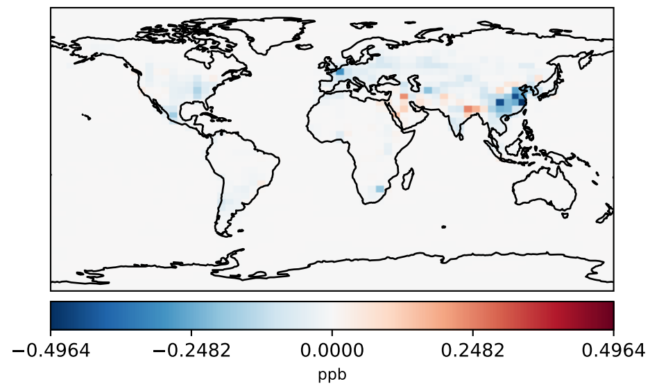
gcc-4x5-1Mon-14.4.0-alpha.1 - gcc-4x5-1Mon-14.4.0-alpha.0 (Ref) 4.0x5.0
