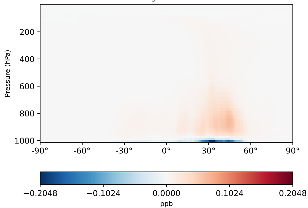
gchp-c24-1Mon-14.4.0-alpha.1 - gchp-c24-1Mon-14.4.0-alpha.0 (Dev) 1x1.25 regridded from c24
