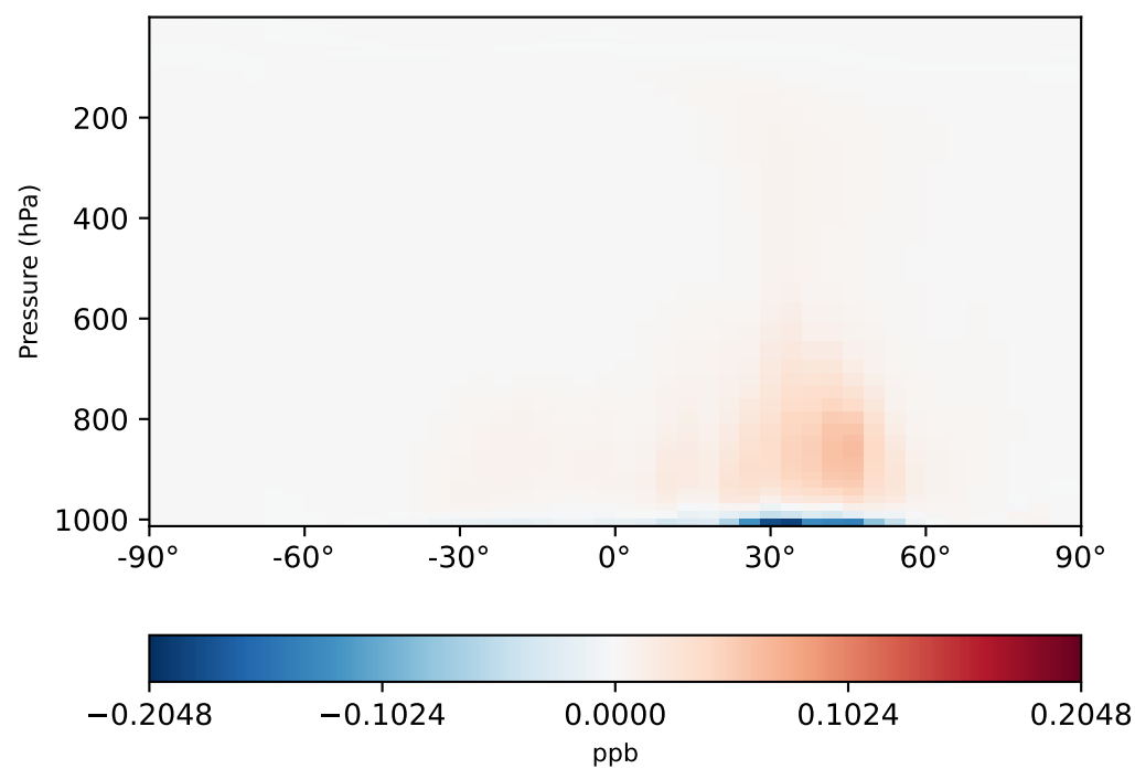
gcc-4x5-1Mon-14.4.0-alpha.1 - gcc-4x5-1Mon-14.4.0-alpha.0 (Ref) 4.0x5.0
