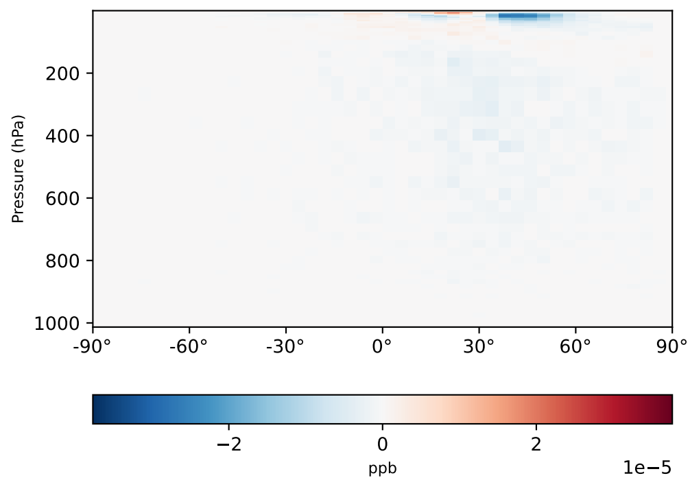
gcc-4x5-1Mon-14.4.0-alpha.1 - gcc-4x5-1Mon-14.4.0-alpha.0 (Ref) 4.0x5.0
