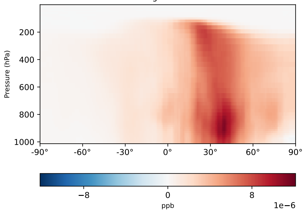
gchp-c24-1Mon-14.4.0-alpha.1 - gchp-c24-1Mon-14.4.0-alpha.0 (Dev) 1x1.25 regridded from c24
