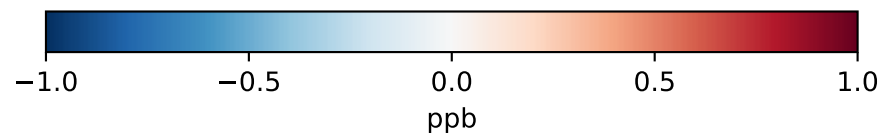
Difference (1x1.25), Restricted Range [5%,95%] \text{GCHP\_dev} / \text{GCHP\_ref} - \text{GCC\_dev} / \text{GCC\_ref}
