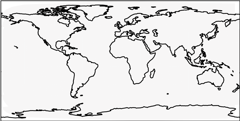
GCHP_dev - GCHP_ref (Dev) c24
