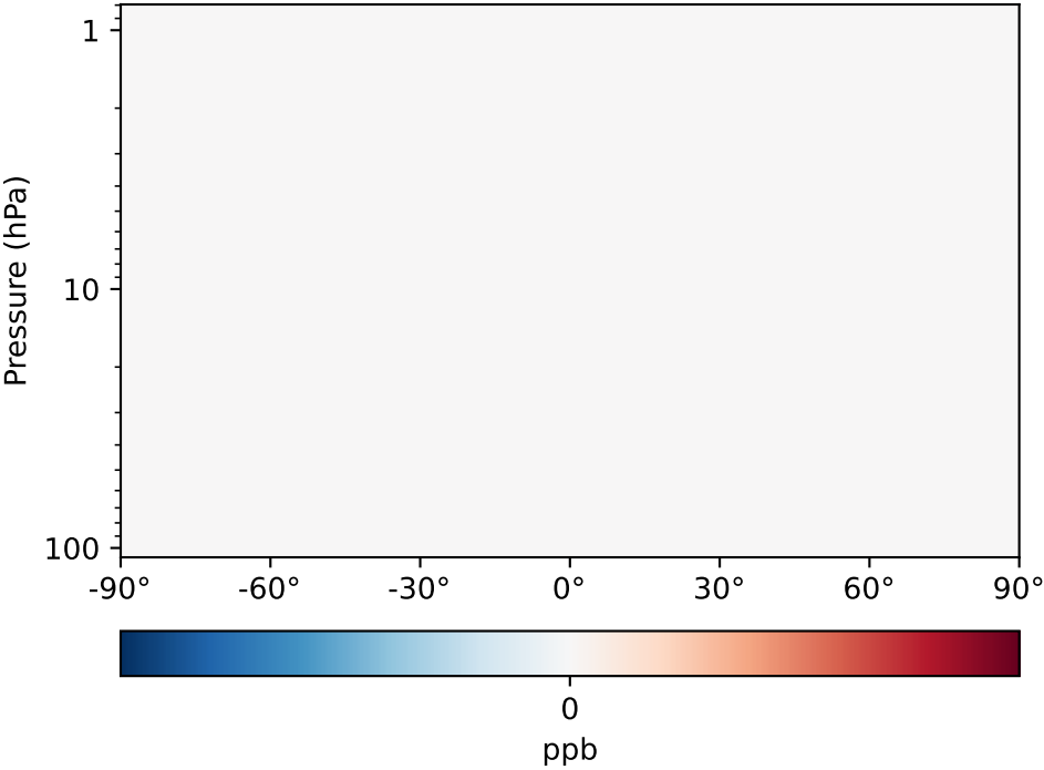
Difference (1x1.25), Dynamic Range \frac{GCHP\_dev}{GCHP\_ref} - \frac{GCC\_dev}{GCC\_ref}
