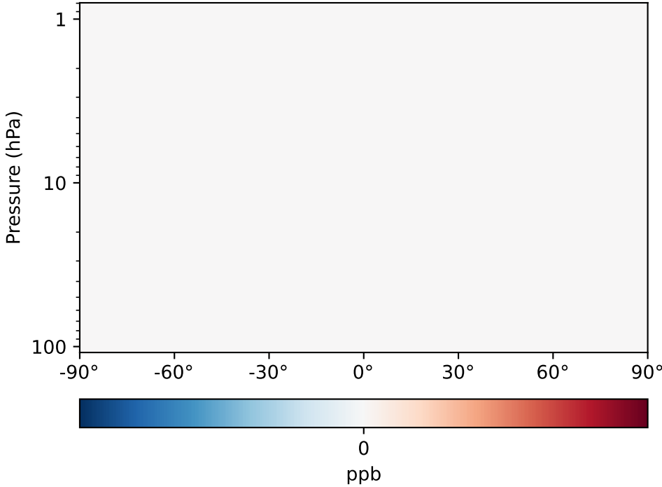
Difference (1x1.25), Restricted Range [5%,95%] \frac{GCHP\_dev}{GCHP\_ref} - \frac{GCC\_dev}{GCC\_ref}
