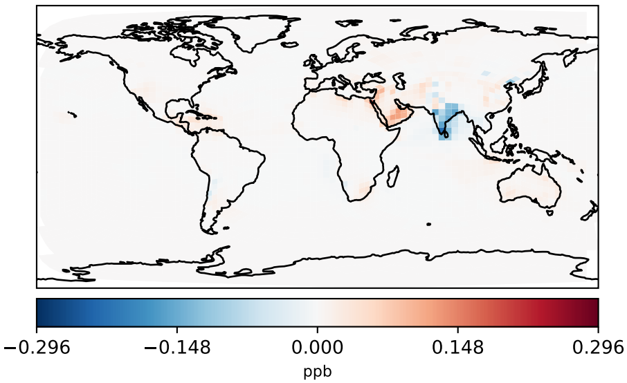
gcc-4x5-1Mon-14.7.0-alpha.17_-_gcc-4x5-1Mon-14.7.0-alpha.16 (Ref) 4.0x5.0 gchp-c24-1Mon-14.7.0-alpha.17_-_gchp-c24-1Mon-14.7.0-alpha.16 (Dev) c24
