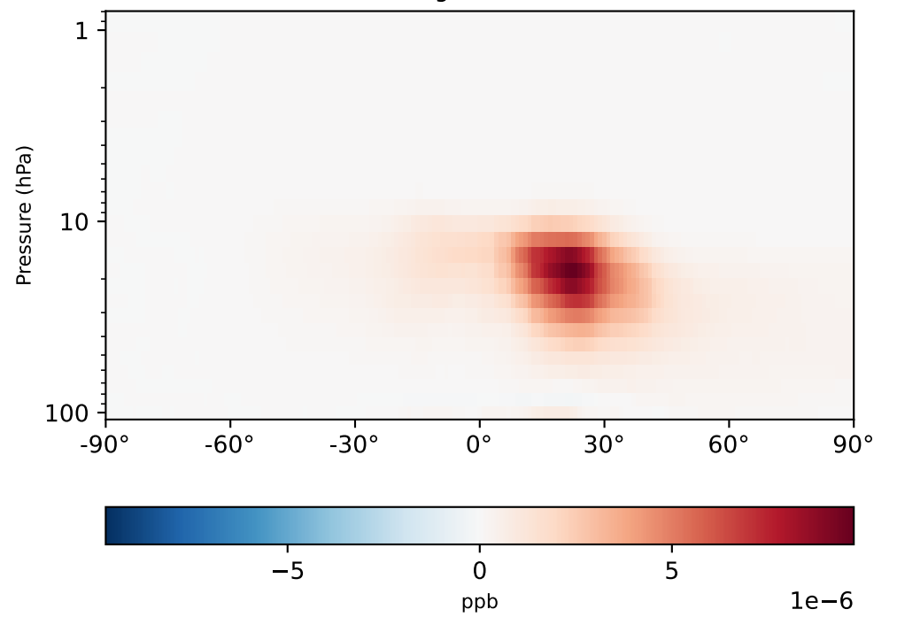
gchp-c24-1Mon-14.7.0-alpha.17 - gchp-c24-1Mon-14.7.0-alpha.16 (Dev) 1x1.25 regrided from c24
