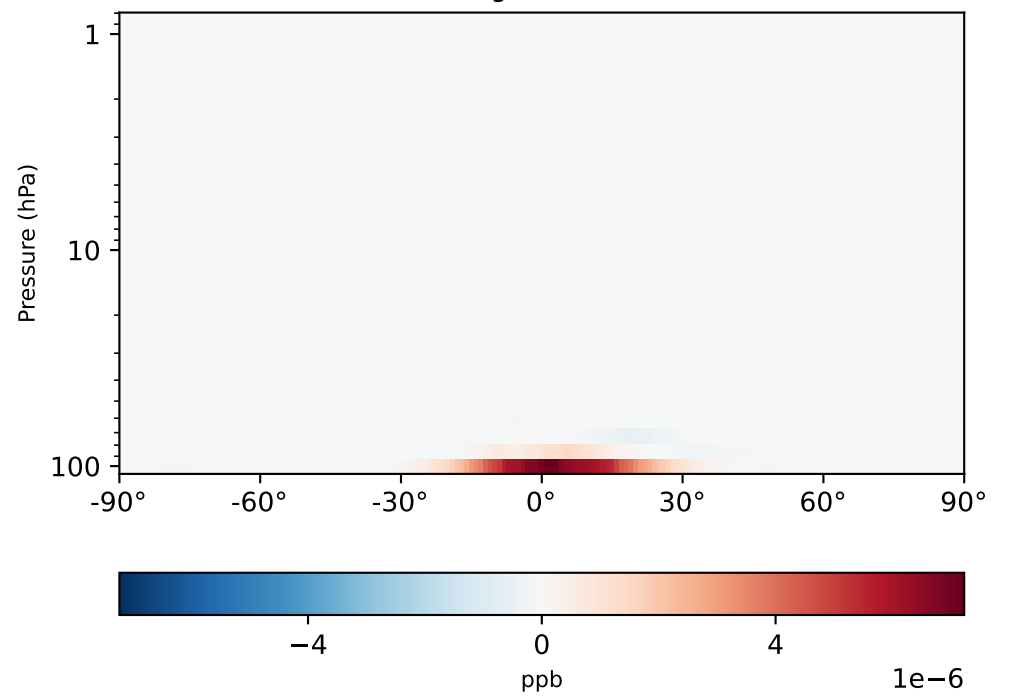
gchp-c24-1Mon-14.7.0-alpha.17 - gchp-c24-1Mon-14.7.0-alpha.16 (Dev) 1x1.25 regridded from c24
