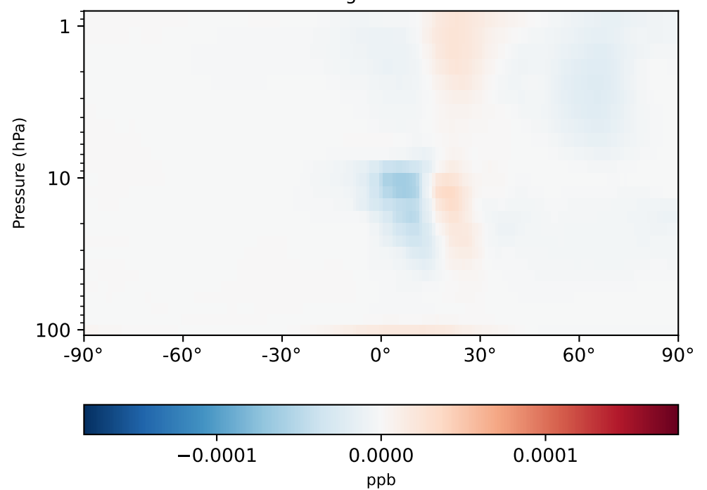
gchp-c24-1Mon-14.7.0-alpha.17 - gchp-c24-1Mon-14.7.0-alpha.16 (Dev) 1x1.25 regridded from c24
