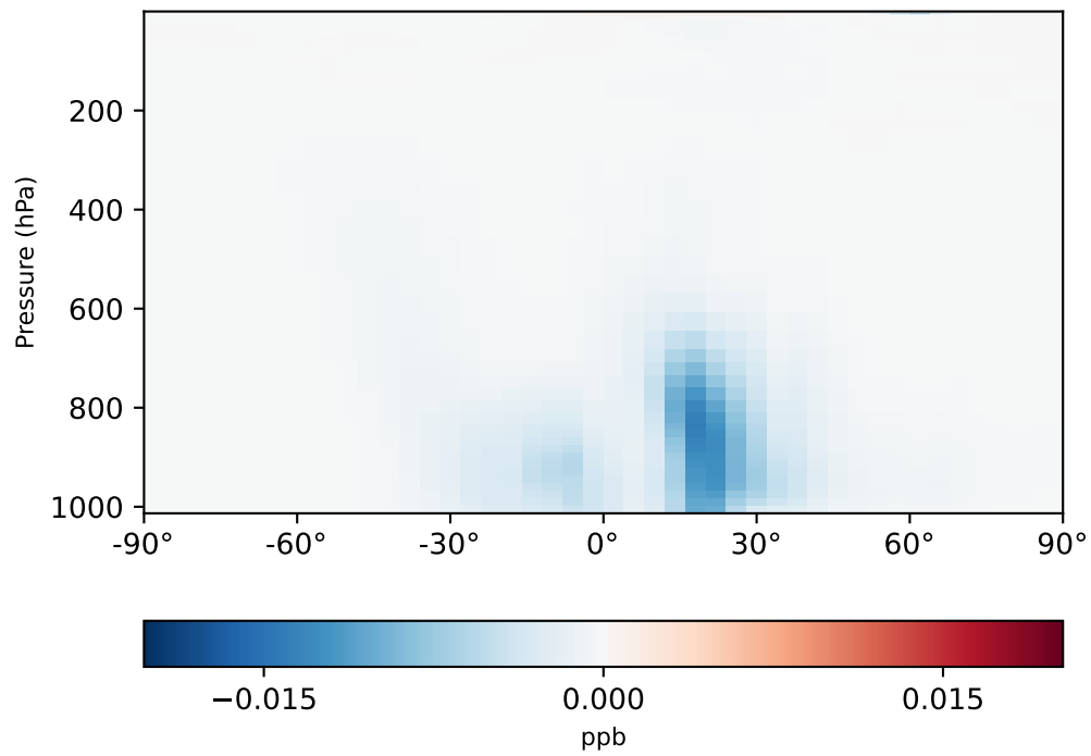
gcc-4x5-1Mon-14.7.0-alpha.17 - gcc-4x5-1Mon-14.7.0-alpha.16 (Ref) 4.0x5.0
