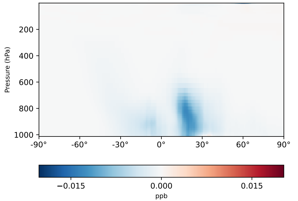
gchp-c24-1Mon-14.7.0-alpha.17 - gchp-c24-1Mon-14.7.0-alpha.16 (Dev) 1x1.25 regridded from c24
