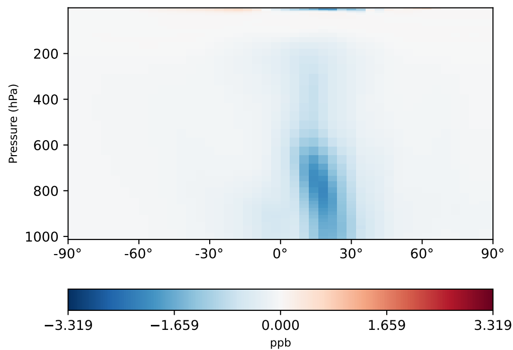
gcc-4x5-1Mon-14.7.0-alpha.17 - gcc-4x5-1Mon-14.7.0-alpha.16 (Ref) 4.0x5.0
